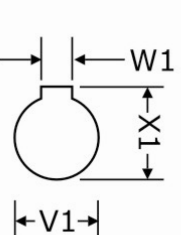
INPUT SHAFT KEYWAY DETAIL
